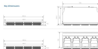
Key dimensions
